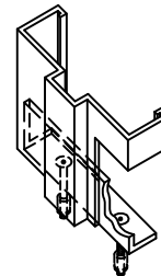
FLOOR ANCHOR FIRE RATED FRAME ANCHOR
